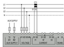
RS485 for DMG7500 and DMG9000
