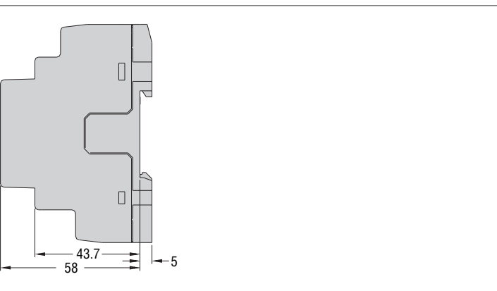
DIMENSIONS MECANQUES [mm]
