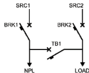
CASE C: 2S – 1T – SI
