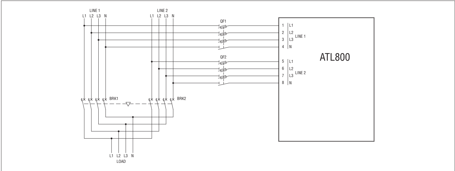
POWER DIAGRAM WITH BREAKERS
