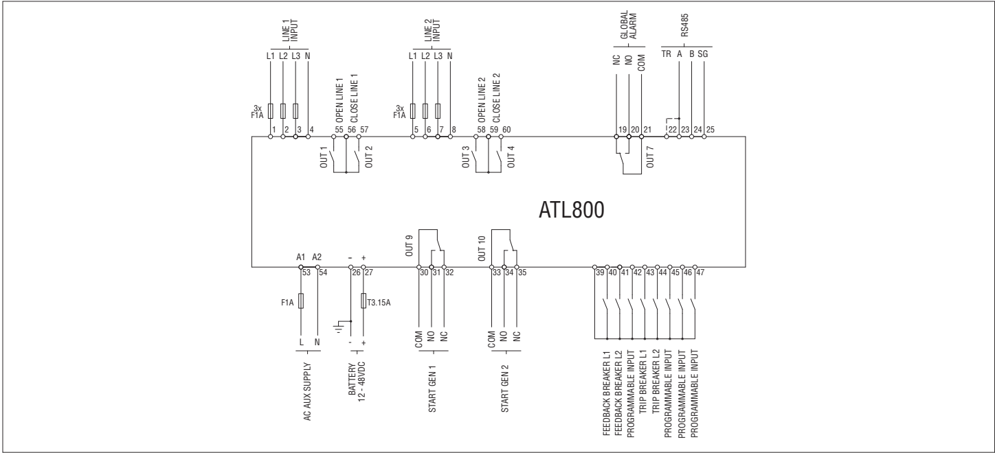
POWER DIAGRAM WITH BREAKERS
