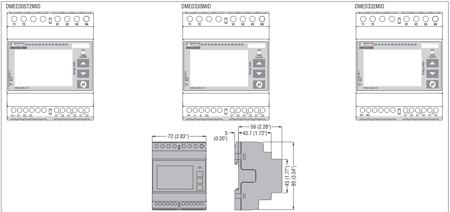
TERMINAL ARRANGEMENT AND MECHANICAL DIMENSIONS [mm (in)]
