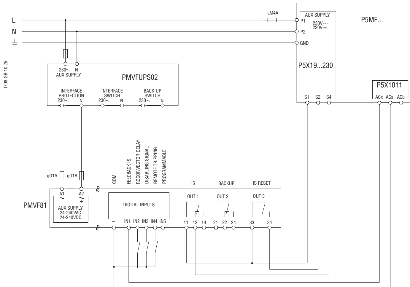
EXAMPLE 6: Configuration with two separate outputs controlling the opening and closing of molded case circuit breakers with impulsive control.
