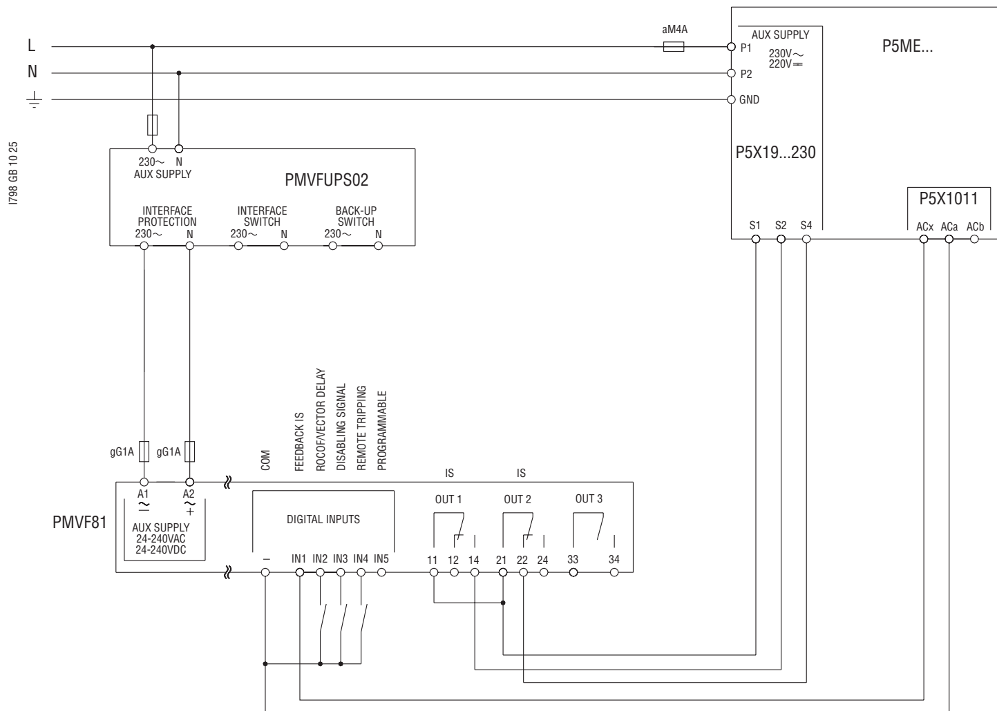
EXAMPLE 3: Configuration with two separate outputs controlling opening and closing.
