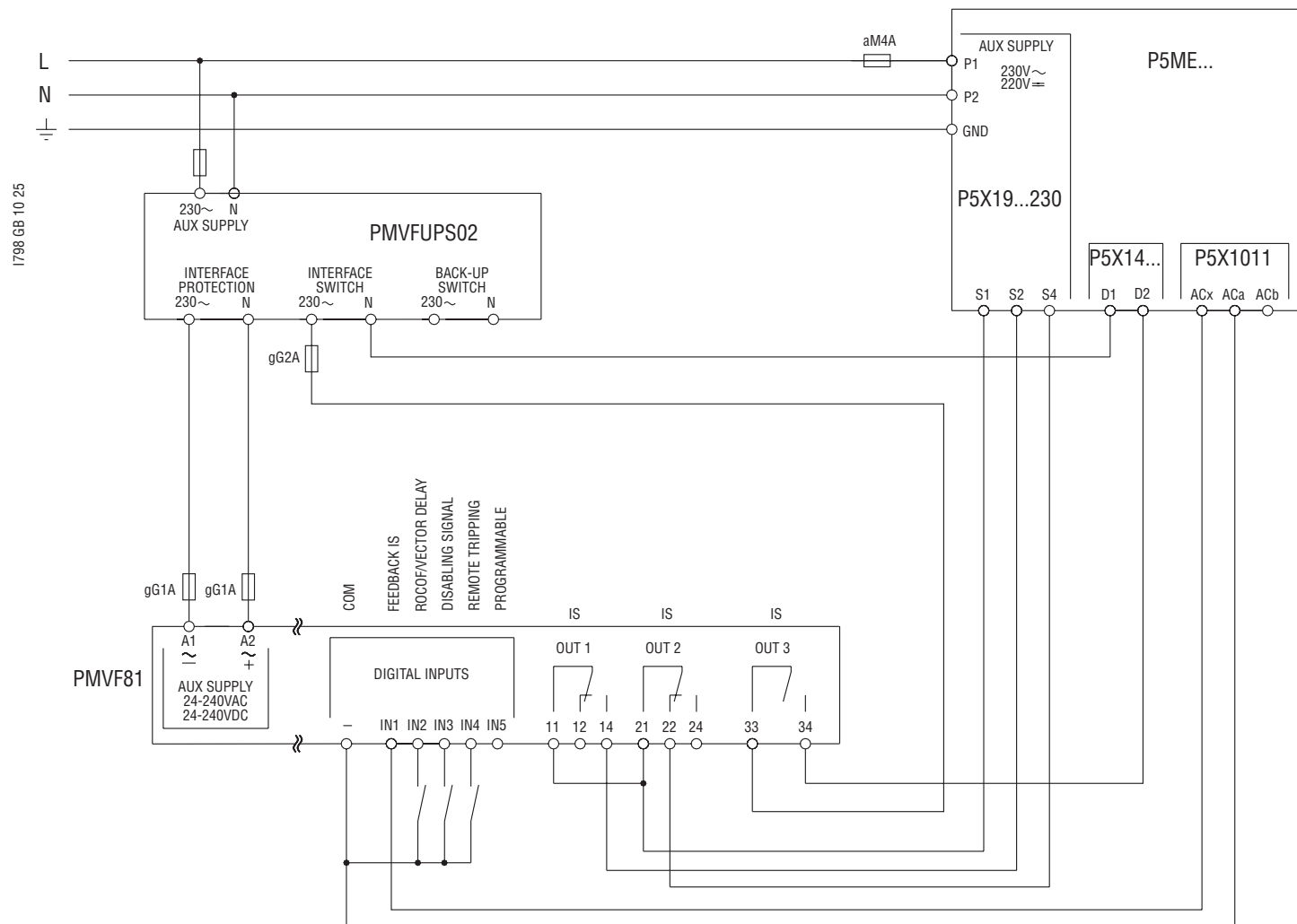
EXAMPLE 4: Configuration with two separate outputs controlling opening and closing and another output (OUT3) for managing the minimum voltage coil.
