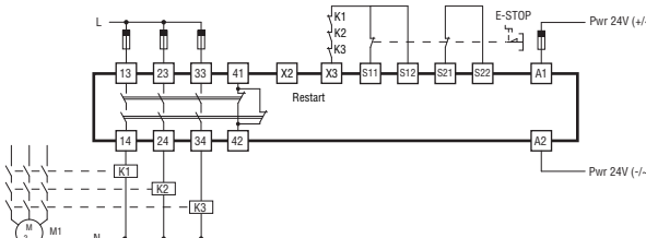
Example of connection of the SRCES31 in MANUAL operation
