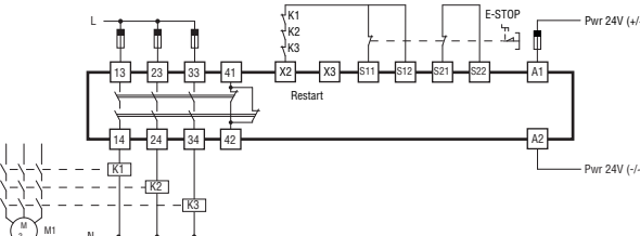
Example of connection of the SRCES31 in AUTOMATIC operation
