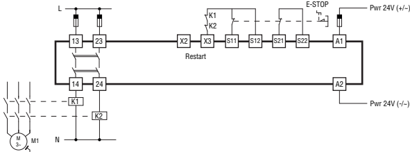
Example of connection of the SRCES20 in MANUAL operation
