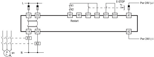
Example of connection of the SRCES20 in AUTOMATIC operation
