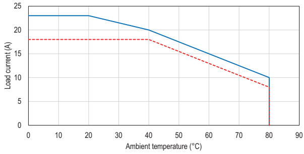
HS3C...020...
