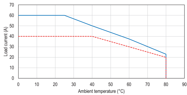
HS1C...060...
