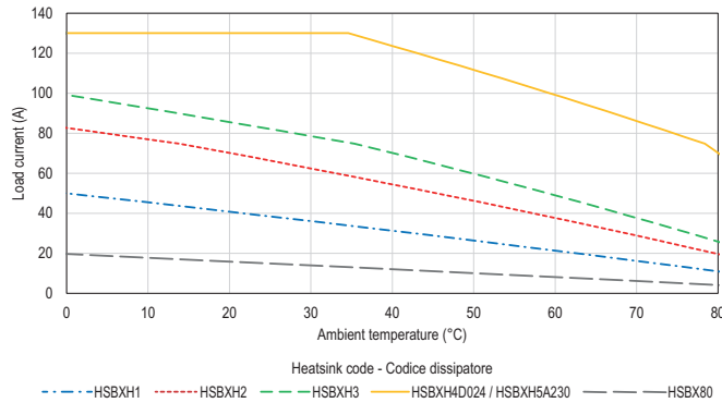
HS1B...130...
