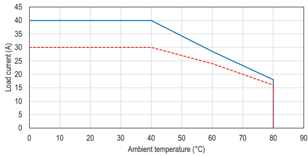
HS3C...040...
