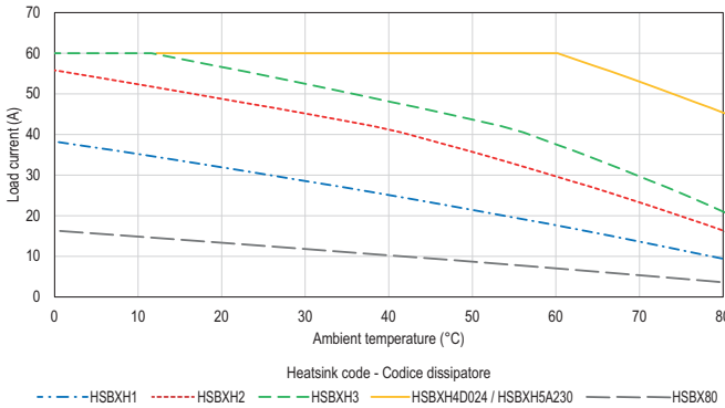
HS1B...060...
