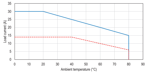
HS1C...025...
