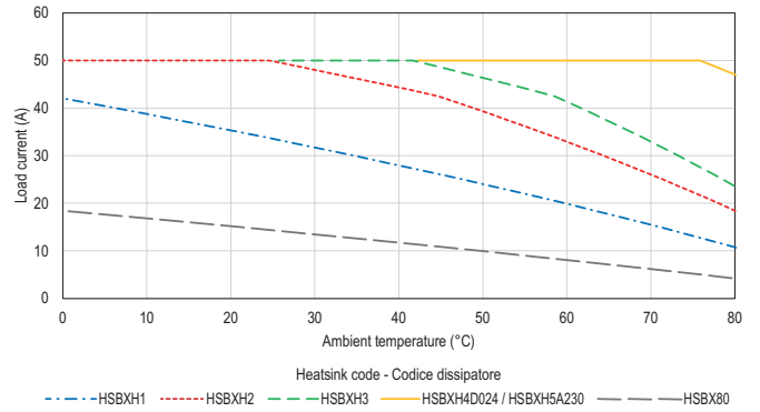
HS1B6NN050D024
