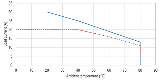
HS3C...025...
