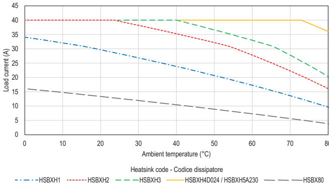
HS1B...040...
