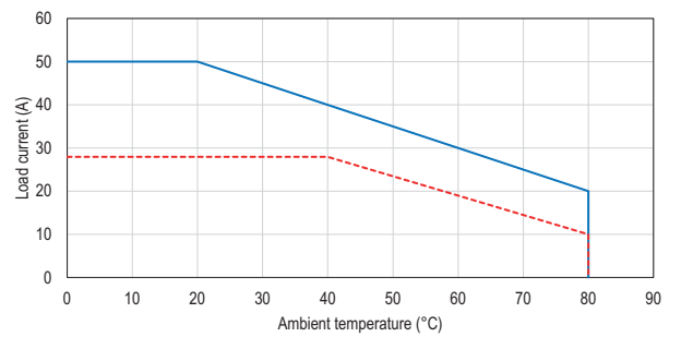
HS1C...040...
